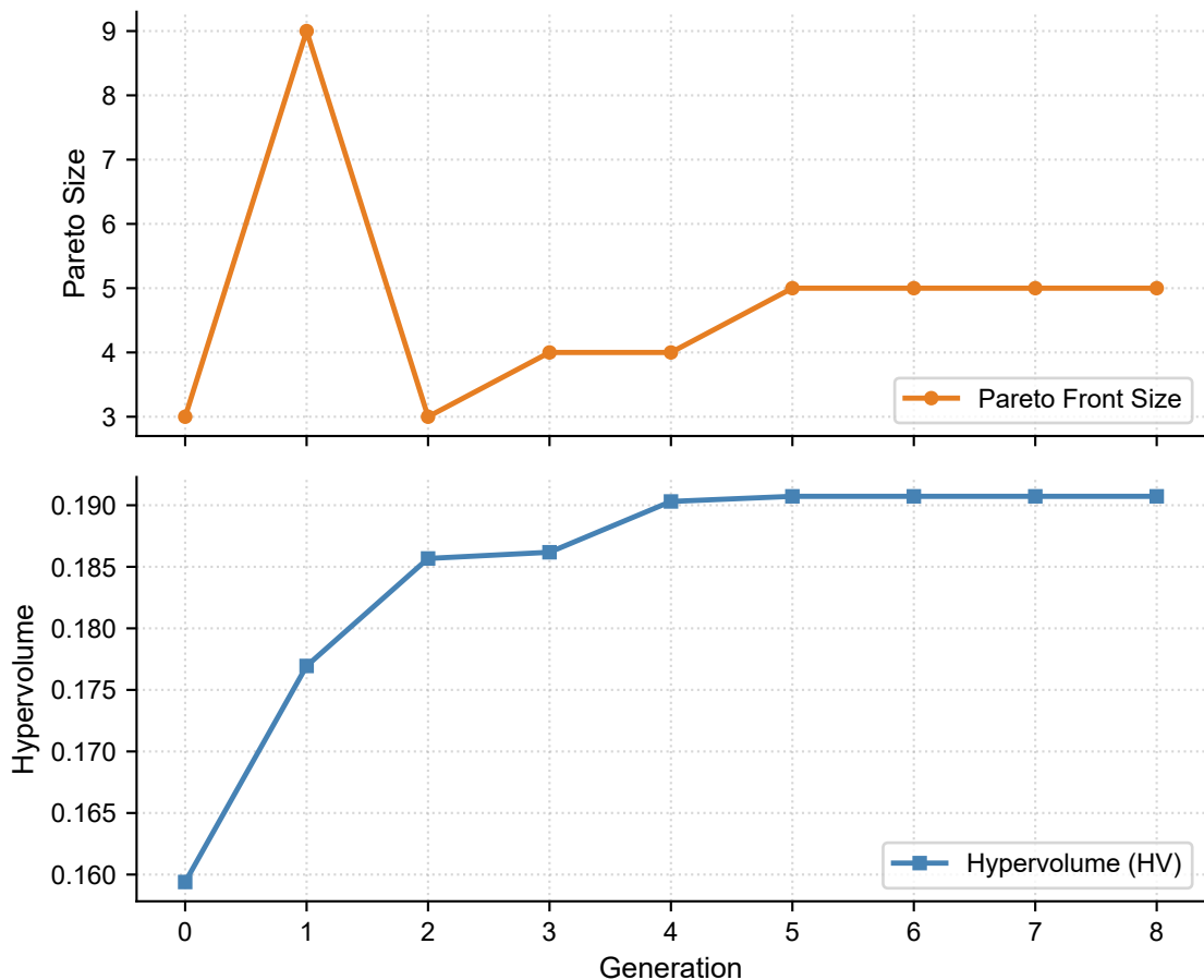
(c) Performance Metrics over Generations
